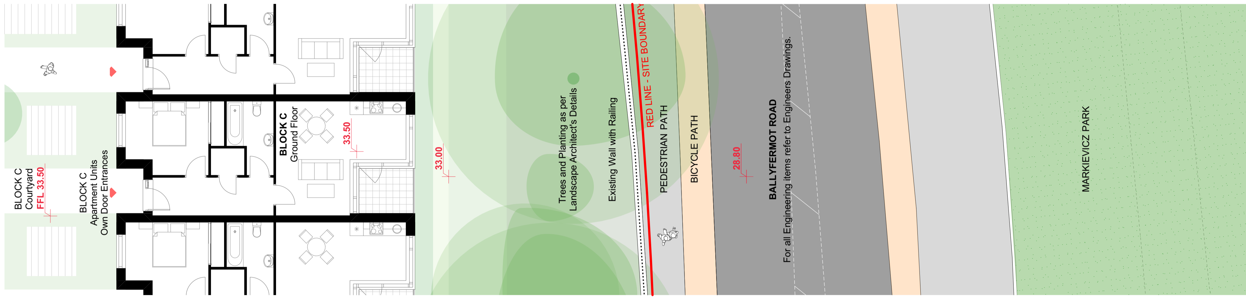
BOUNDARY CONDITION PLAN S03 - BLOCK C / BALLYFERMOT ROAD @ GROUND FLOOR LEVEL 1:100
