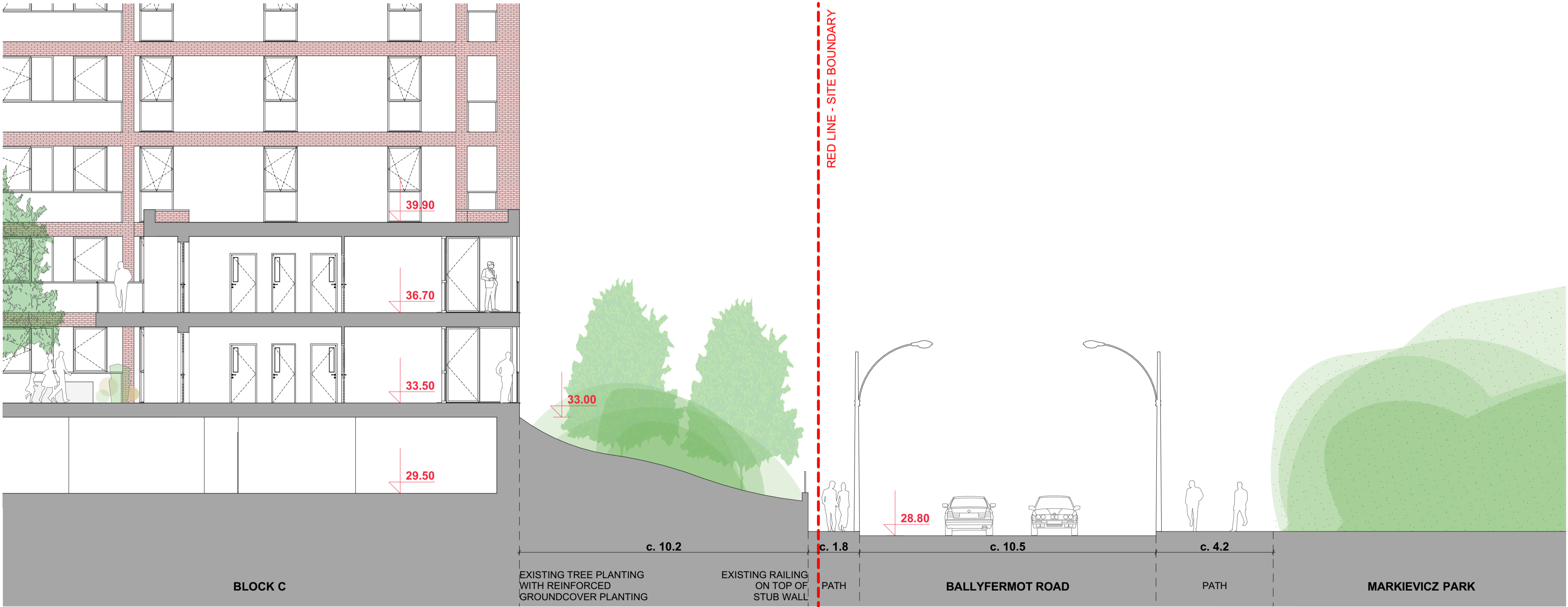
BOUNDARY CONDITION SECTION S03 - BLOCK C / BALLYFERMOT ROAD 1:100
