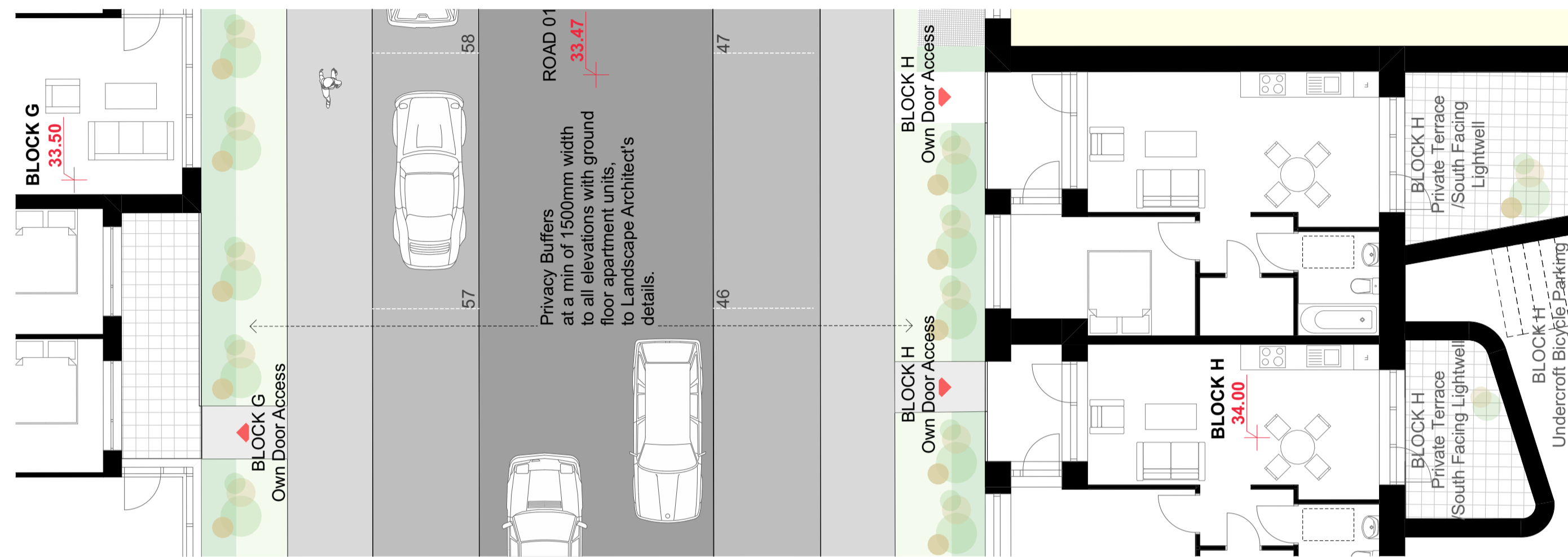
BOUNDARY CONDITION PLAN S08 - BLOCK G / BLOCK H @ GROUND FLOOR LEVEL 1:100
