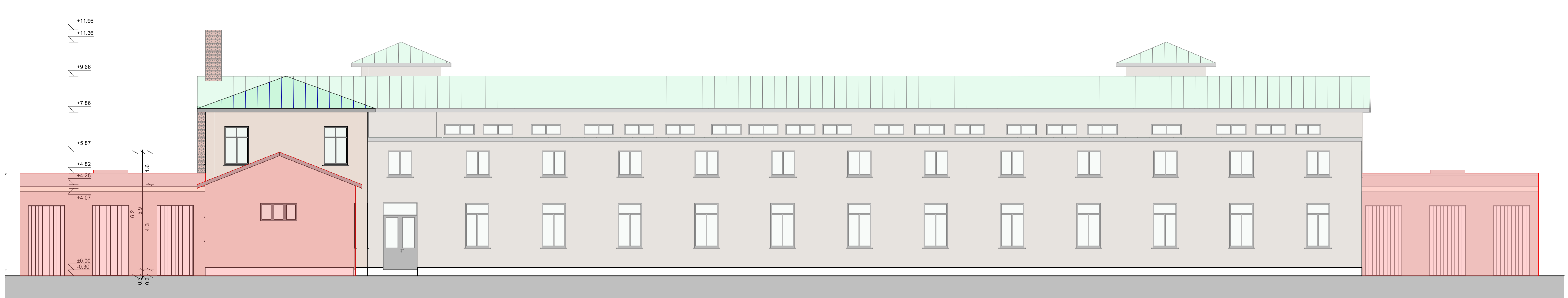
North/Rear Elevation - Demolition 1:100
